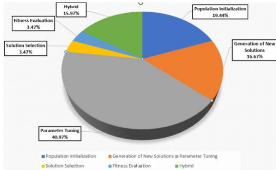
Figure 1. Distribution of ML integration across the operational stages of metaheuristics
